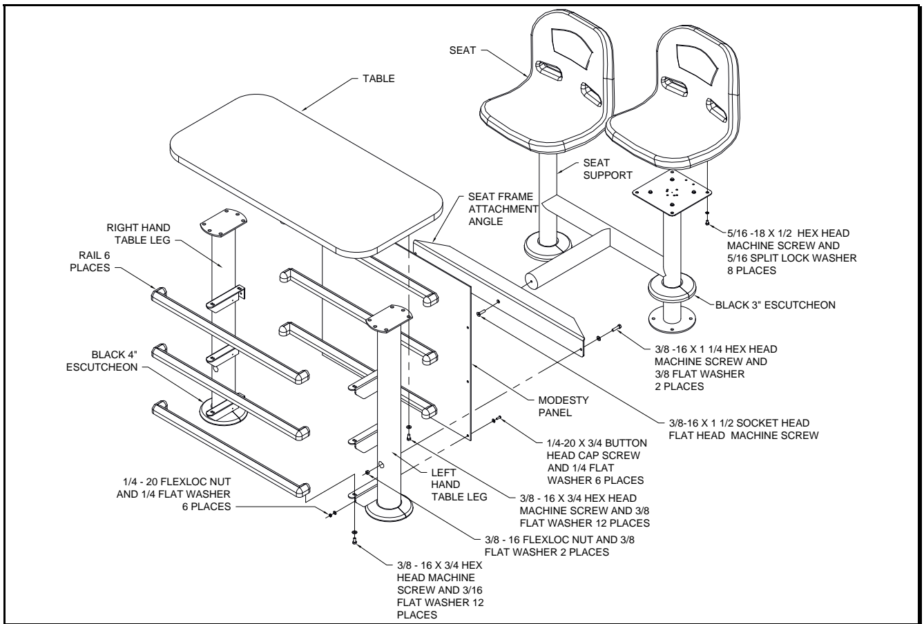
Assembly Exploded View
