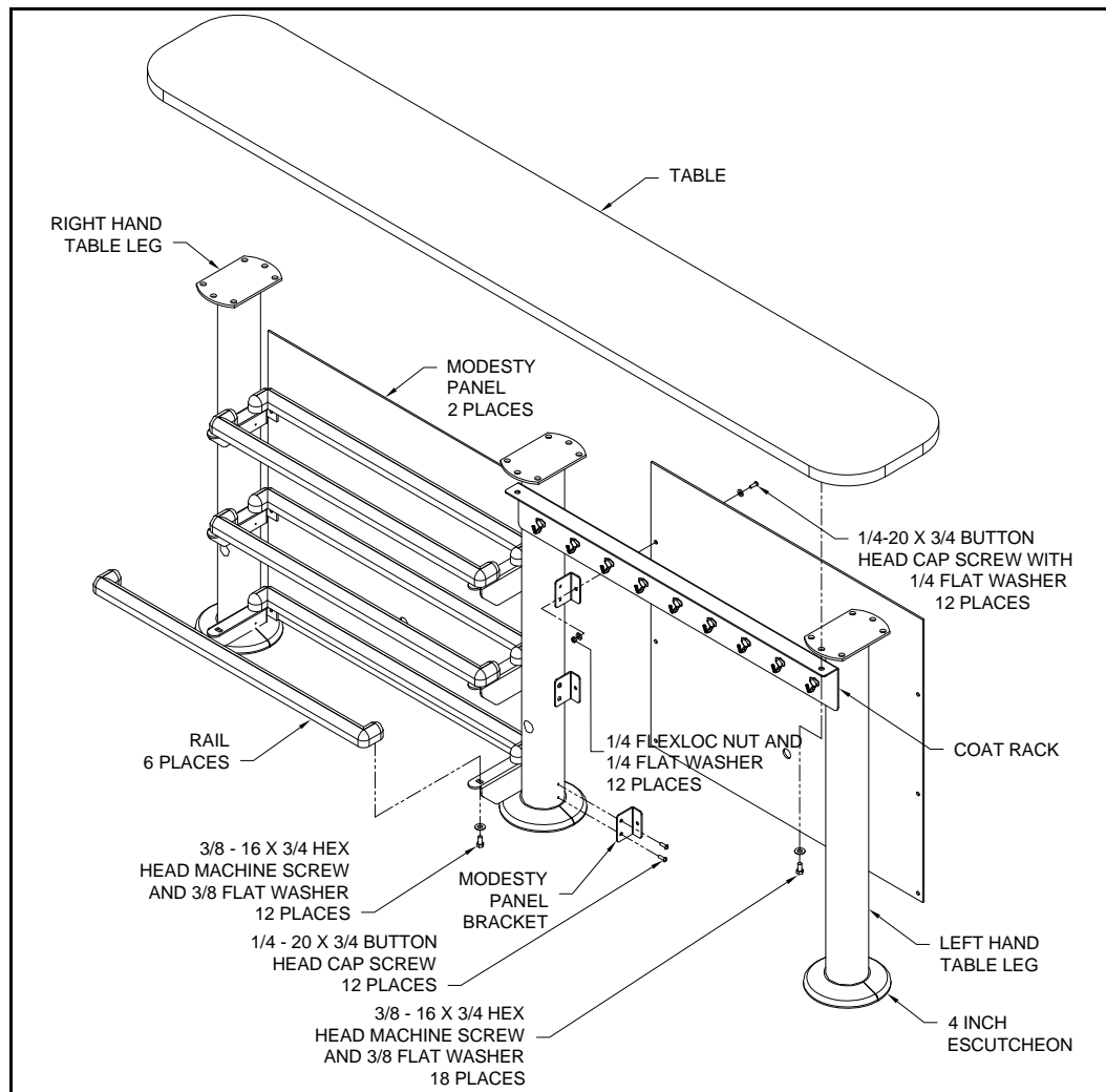
Assembly Exploded View
