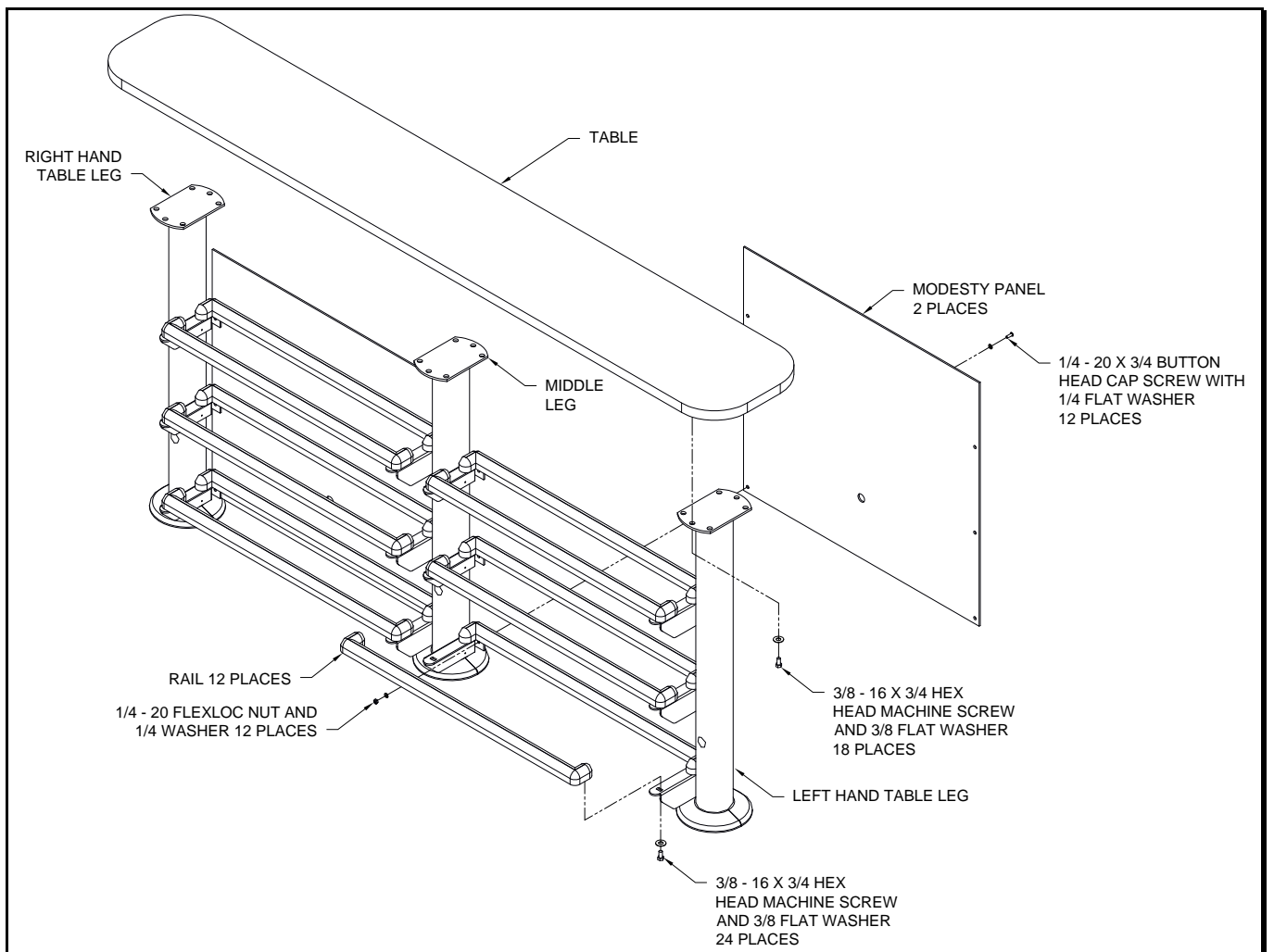
Assembly Exploded View
