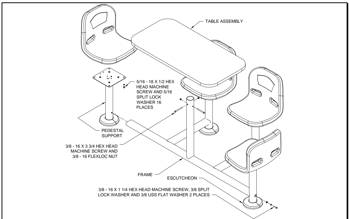
Assembly Exploded View
